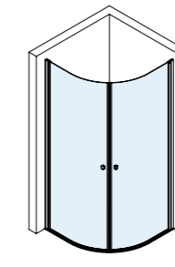
Kwartrond 90x90x200 cm (873-888x873-888 mm) 100x100x200 cm (973-988x973-988 mm)
