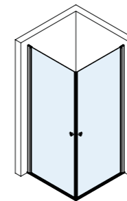
Hoekinstap 90x90x200 cm (873-888x873-888 mm) 100x100x200 cm (973-988x973-988 mm)
